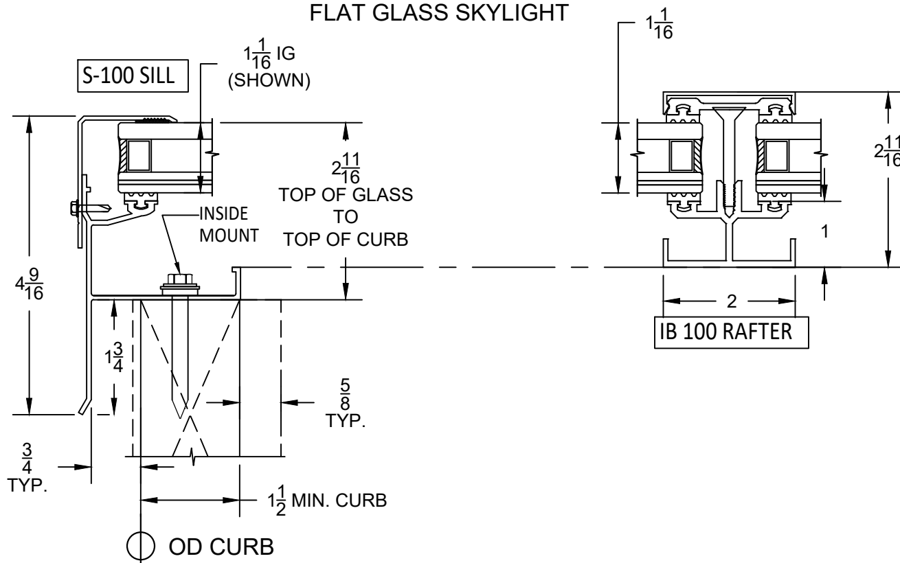
STANDARD SILL @ RAKE END
