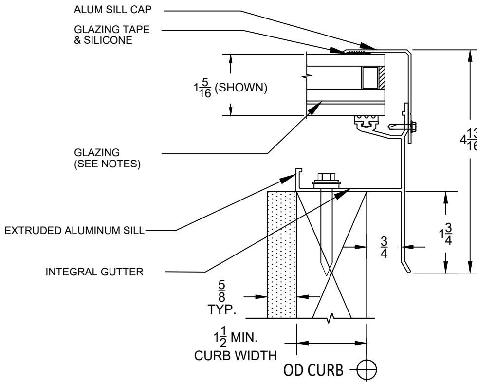
SILL AT RAKE / SIDE S100
