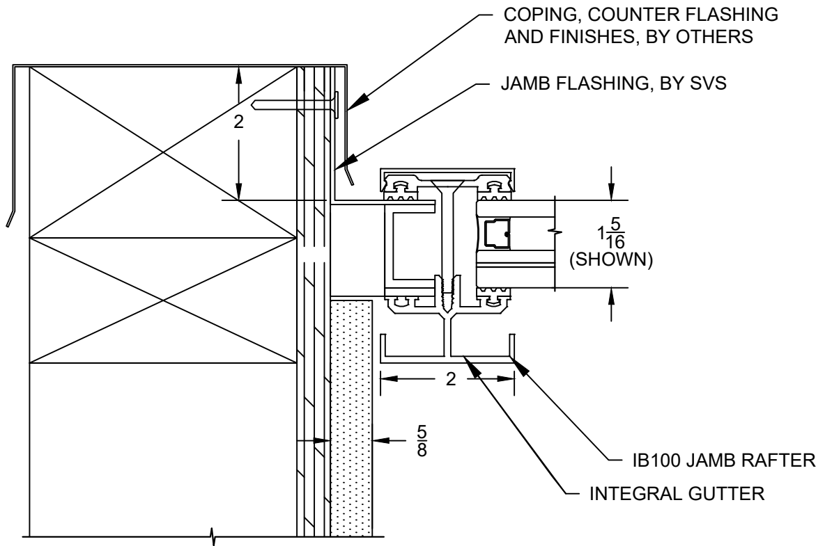
TYPICAL JAMB DETAIL - IB100
